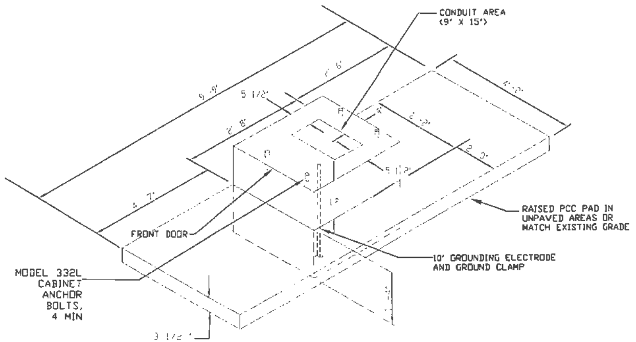
332L FOUNDATION DETAILS
