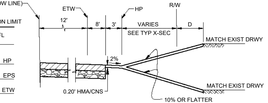
SPECIAL DRIVEWAY APPROACH WITH GRADE MATCH
