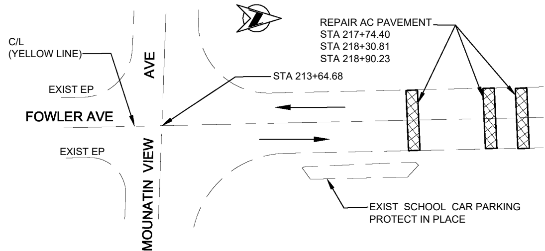
ASPHALT PAVEMENT REPAIR (DIG-OUT)
