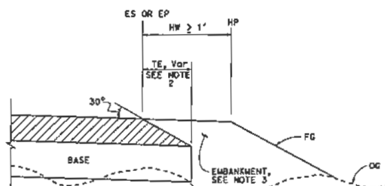
CASE K Tapered Edge - Fill Section, HW \geq 1'
