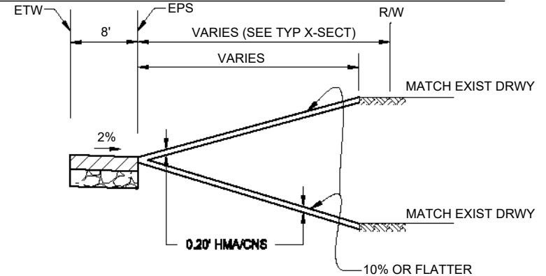
SPECIAL DRIVEWAY APPROACH
