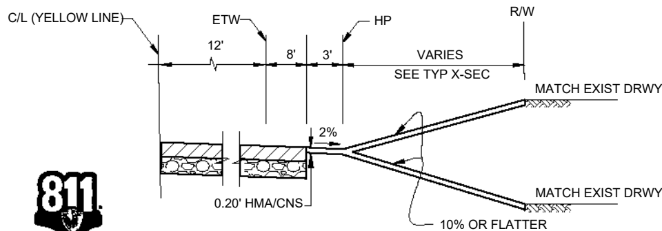
TYPICAL DRIVEWAY APPROACH
