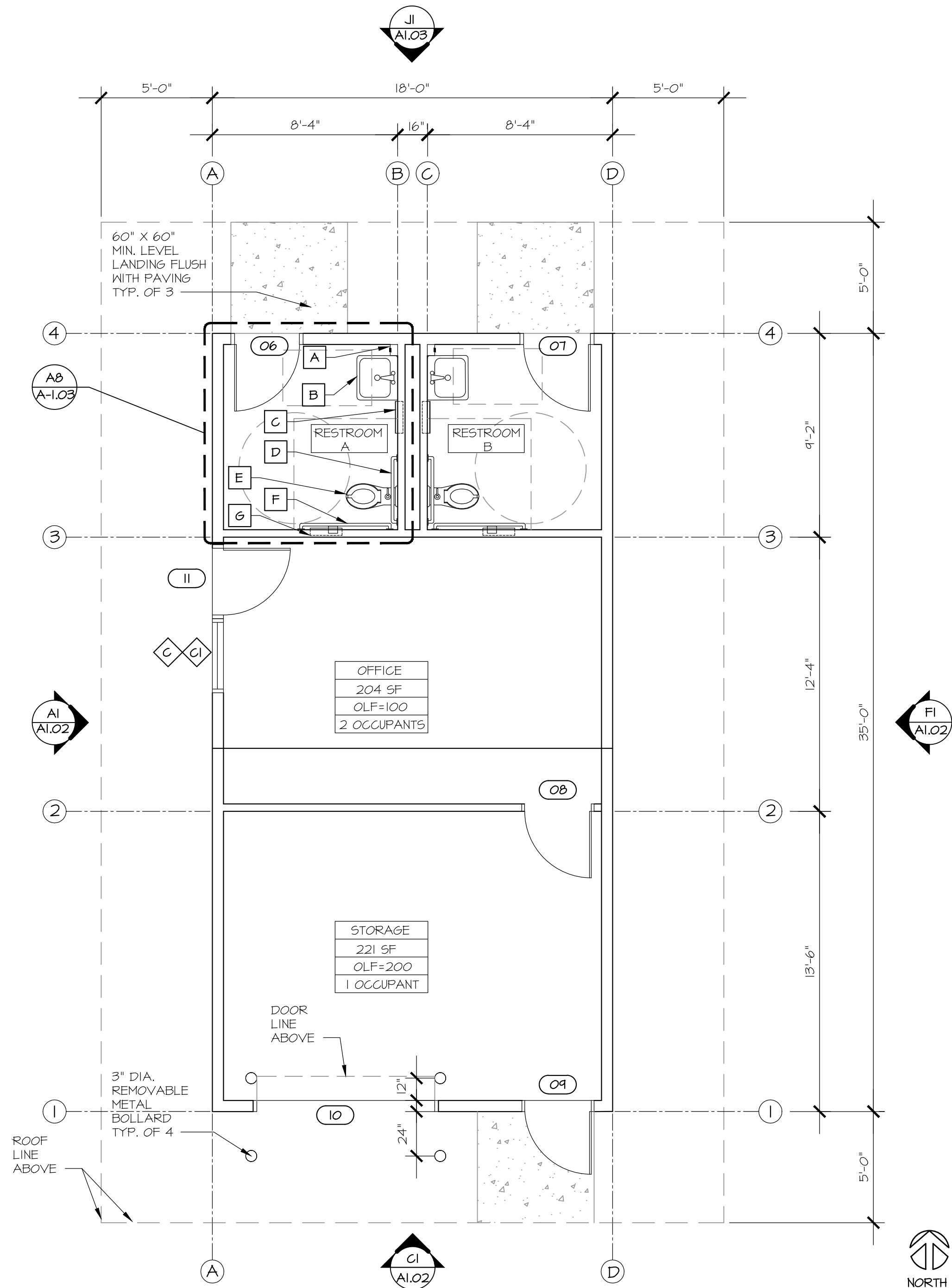
D8 Facility Office Building - Floor Plan Scale: 1/4" = 1'-0"
