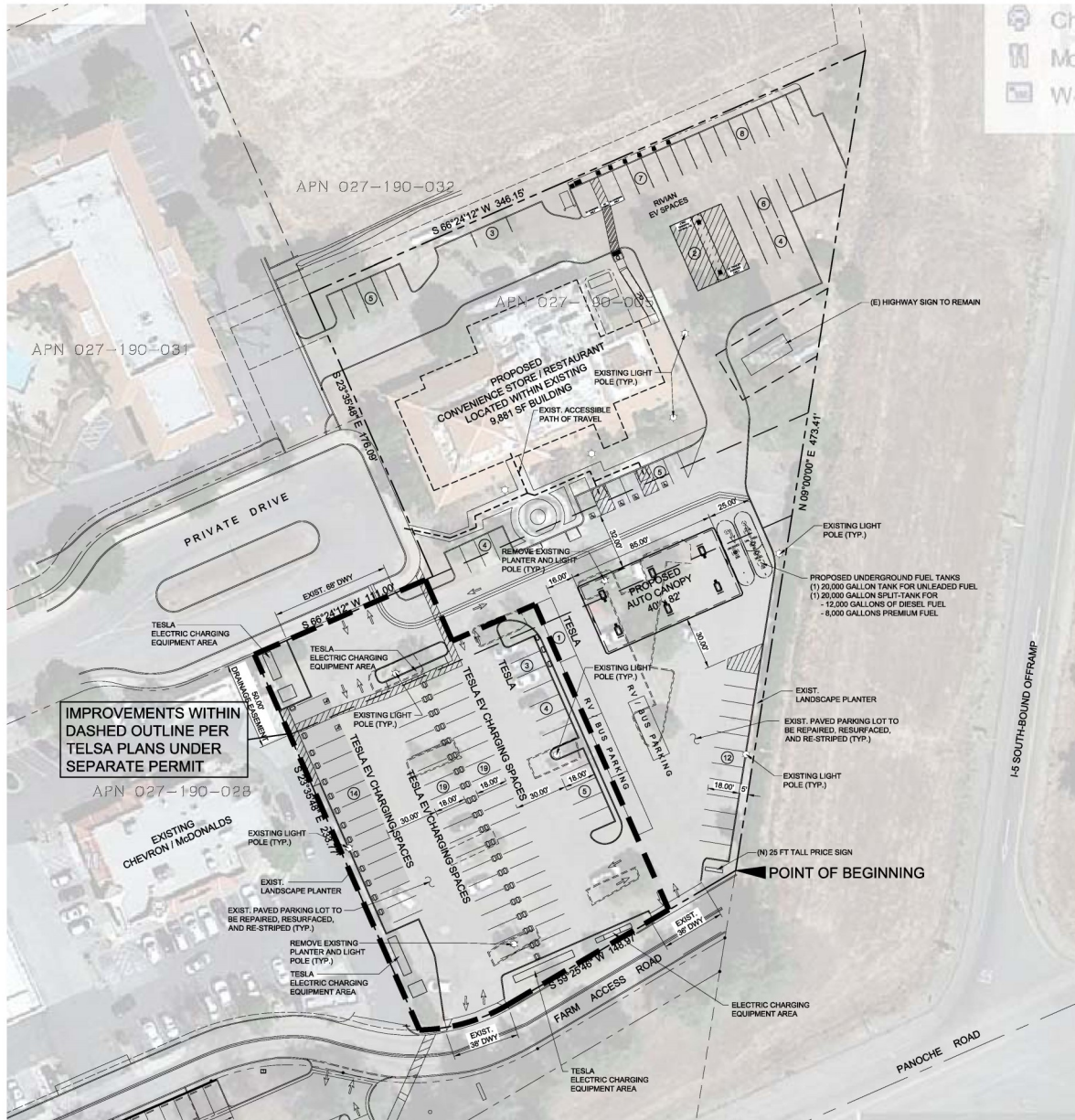
PLOT PLAN
