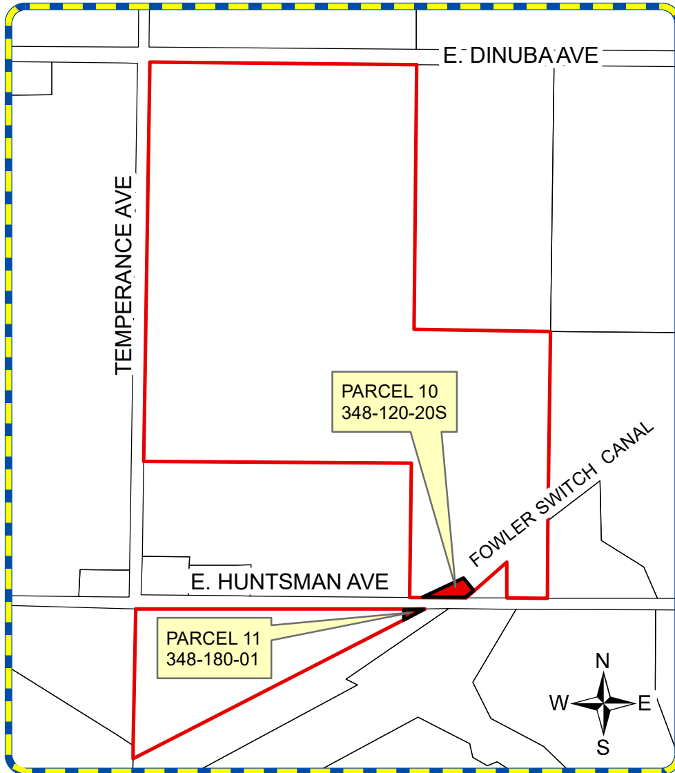
FOWLER SWITCH CANAL BRIDGE AT HUNTSMAN AVE.
