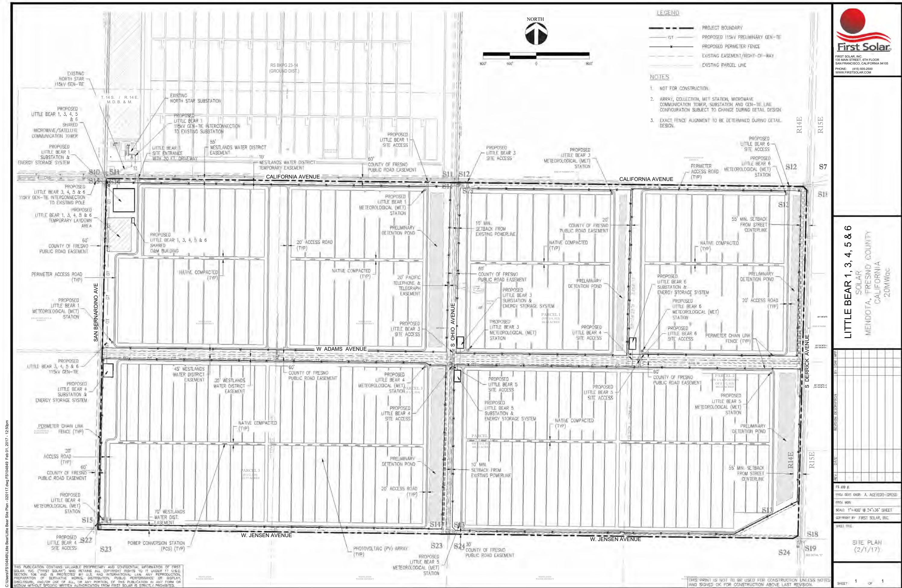
FIGURE 3 -- PROJECT LAYOUT
