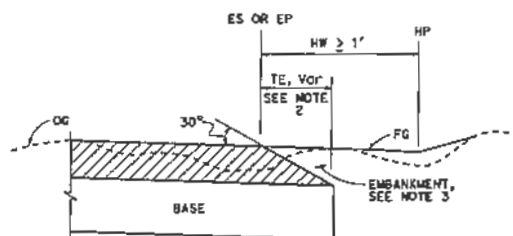
CASE M Tapered Edge - Cut Section, HW \geq 1'
