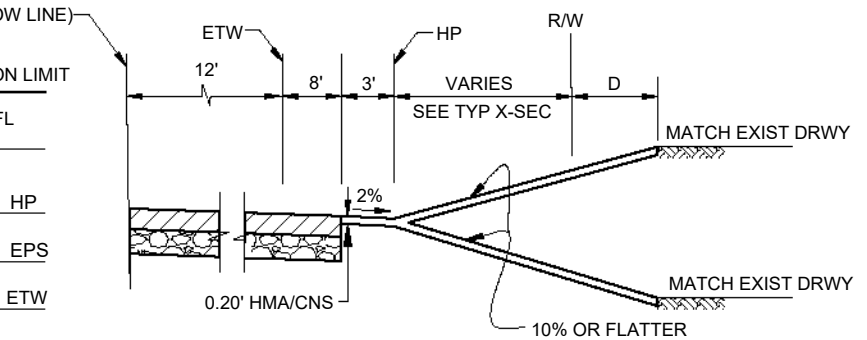
SPECIAL DRIVEWAY APPROACH WITH GRADE MATCH
