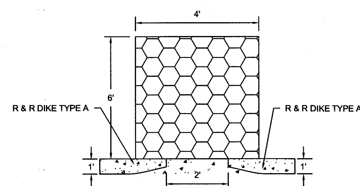
F R & R DIKE TAPERED INLET DETAIL
