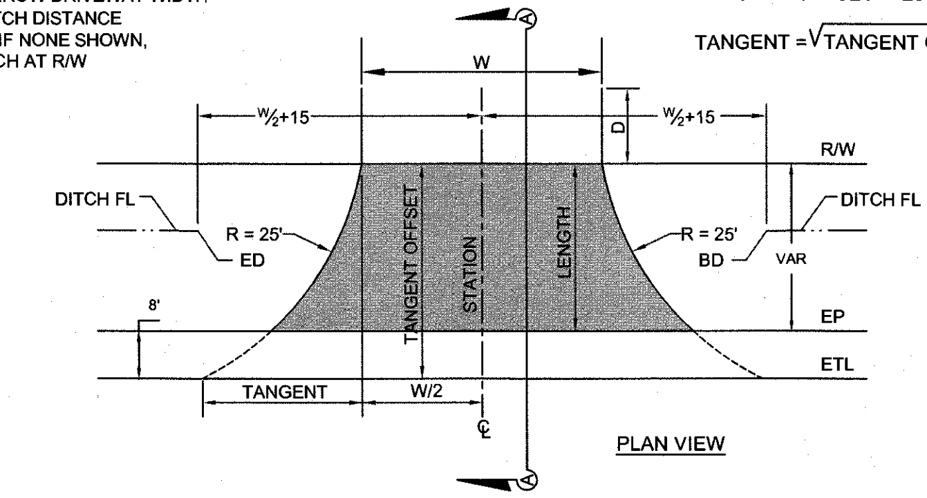
C TYPICAL DIRT DRIVEWAY APPROACH DETAIL NTS
