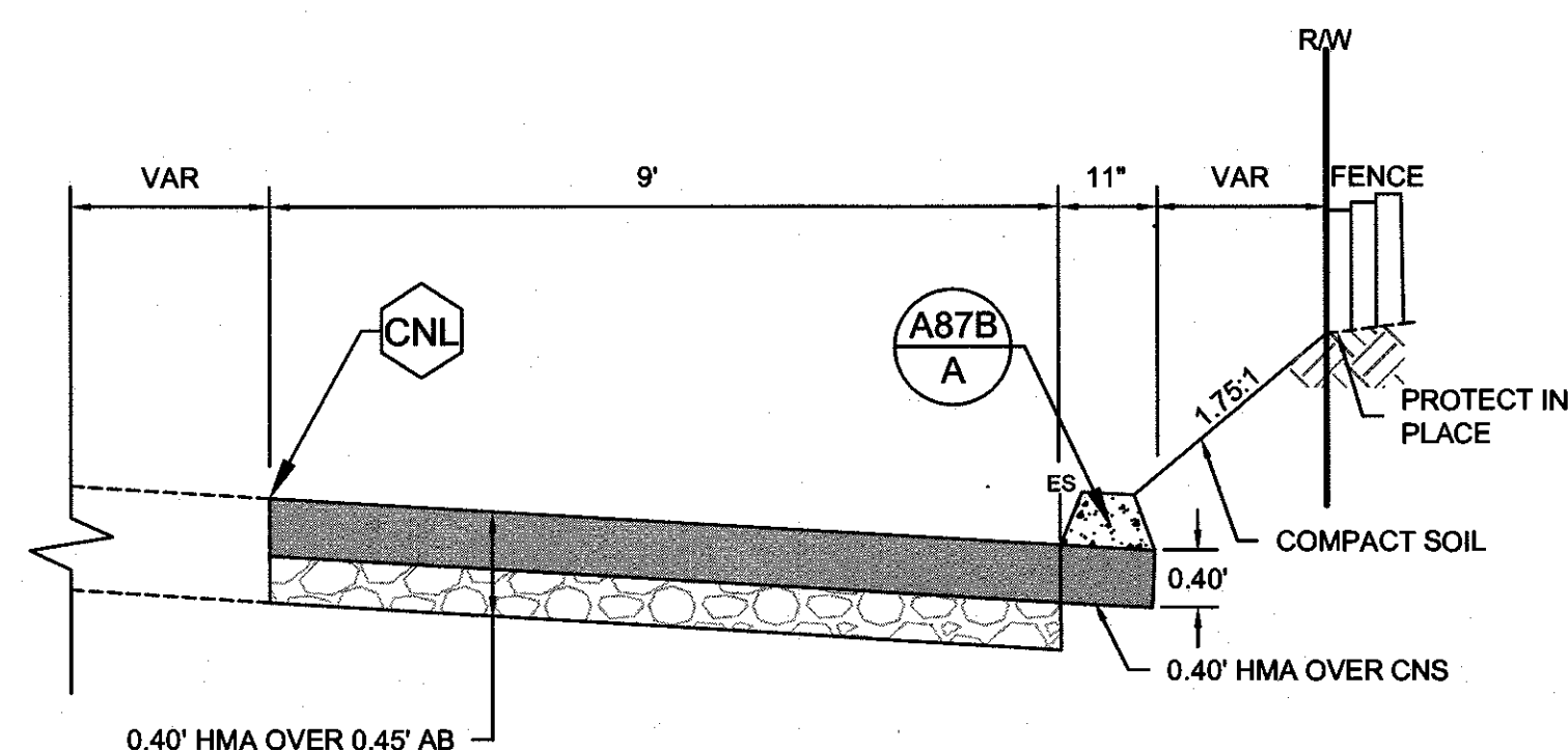
C HMA DIKE TYPE A DETAIL
