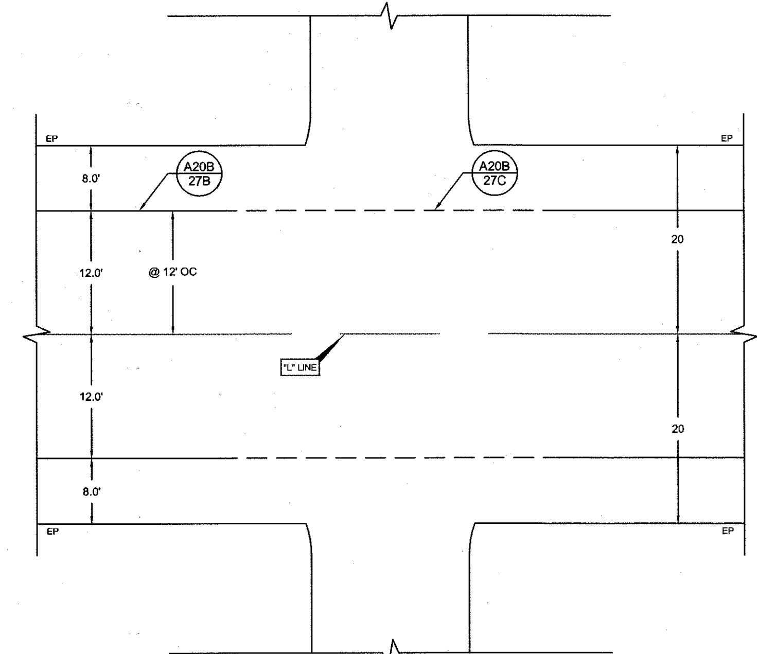
E STRIPING DETAIL NTS
