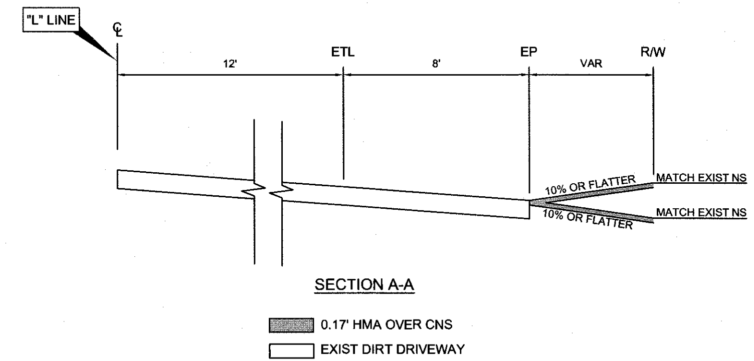
C TYPICAL DIRT DRIVEWAY APPROACH DETAIL NTS
