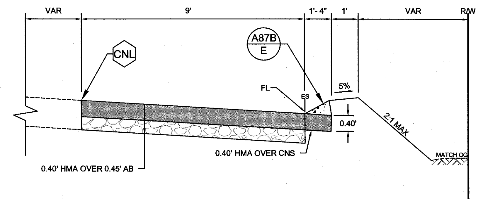
E HMA DIKE TYPE E DETAIL
