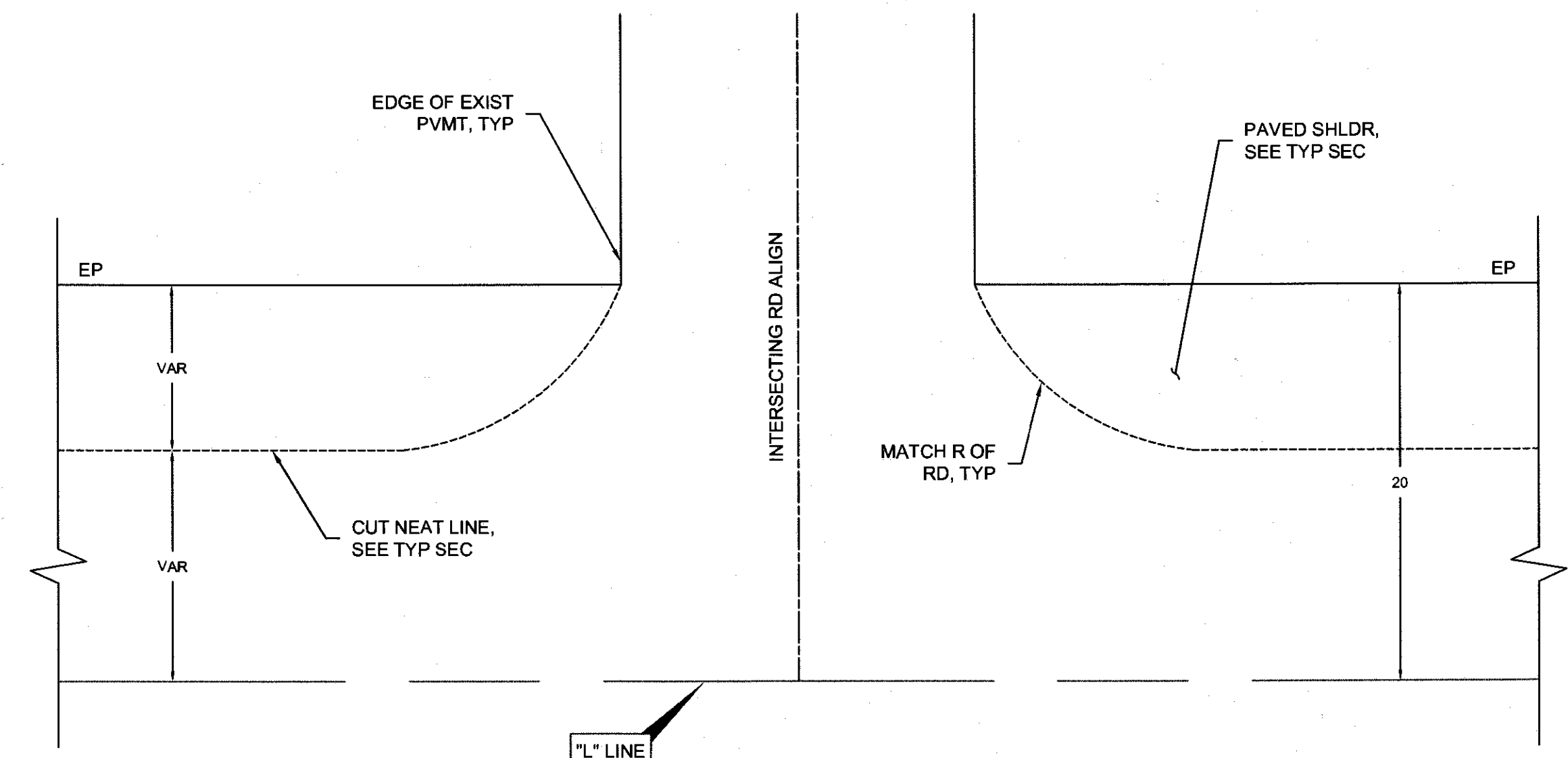
D TYPICAL INTERSECTING ROAD TIE-IN DETAIL NTS
